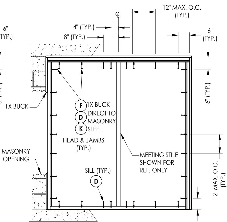
FRAME ANCHORING (1X Buck, Direct to Masonry, Steel Stud)
